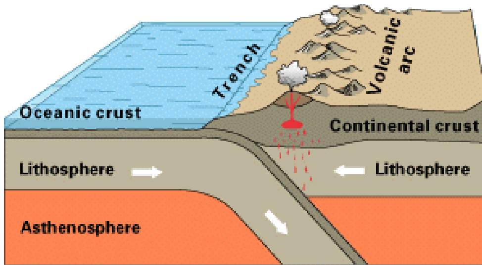
Oceanic-continental convergence
