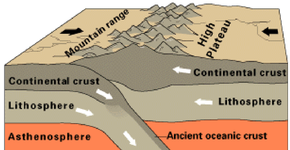
Continental-continental convergence
